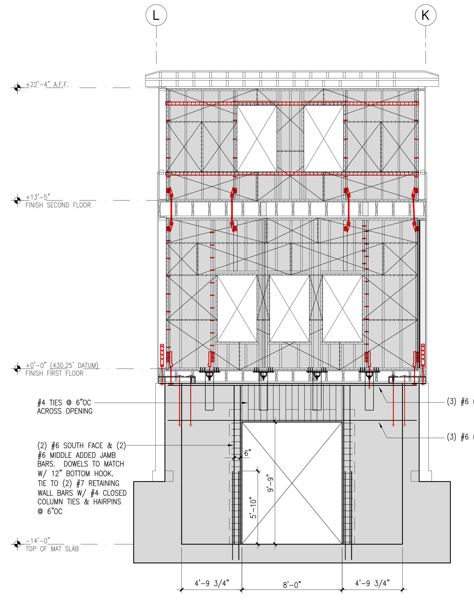
H NORTH INTERIOR WALL ELEV. (GRID 12) 201-SECTS-3 1/4"=1'-0"
