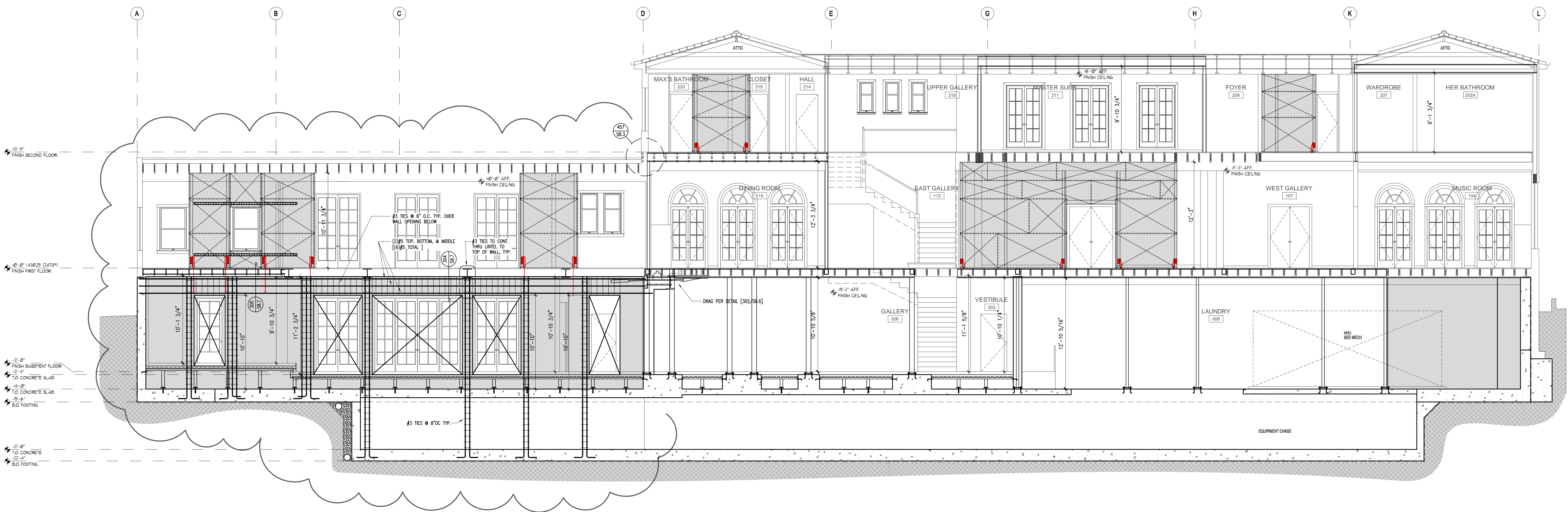
F LONGITUDINAL BUILDING SECTION 201-SECTS-3 3/16"=1'-0"
