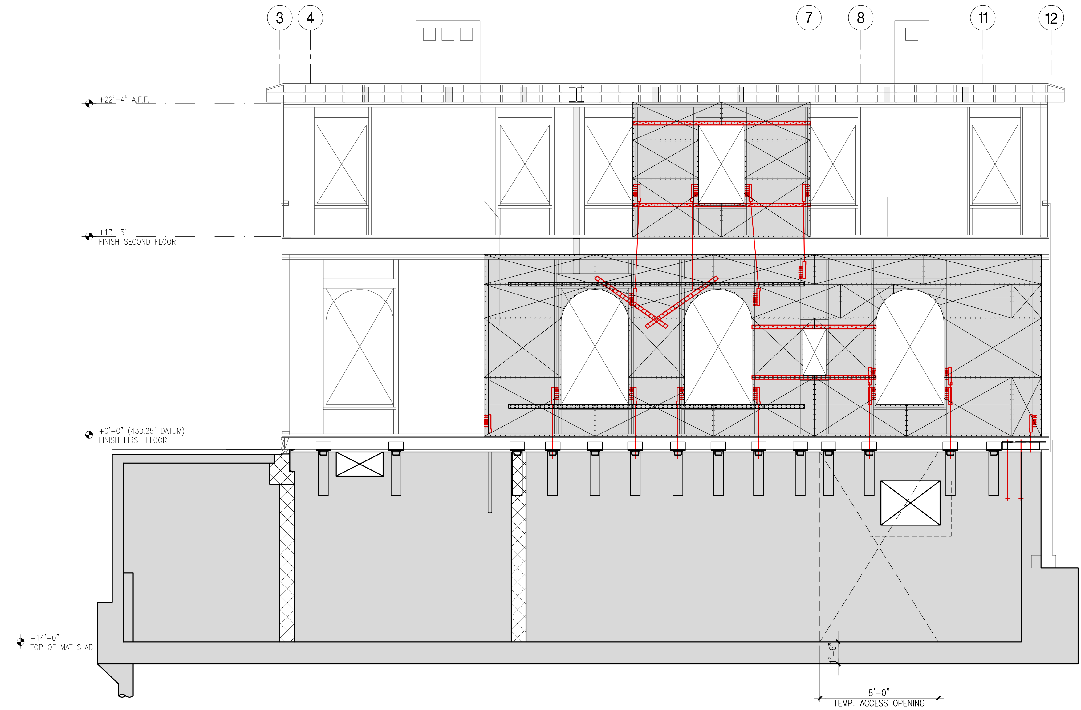
G WEST INTERIOR WALL ELEVATION (GRID L) 201-SECTS-3 1/4"=1'-0"
