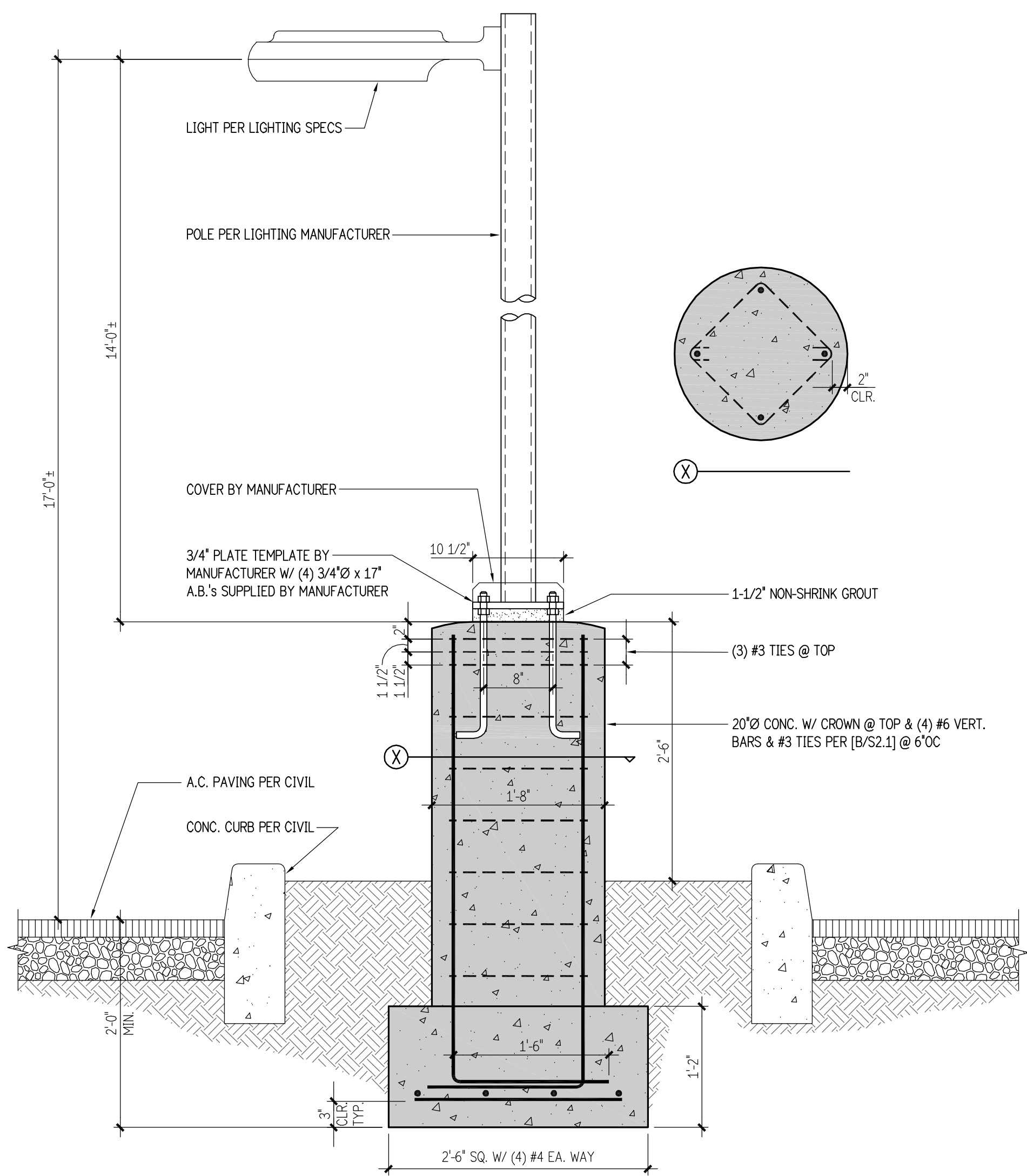
4 LIGHTING BASE 1'-1'-0"
