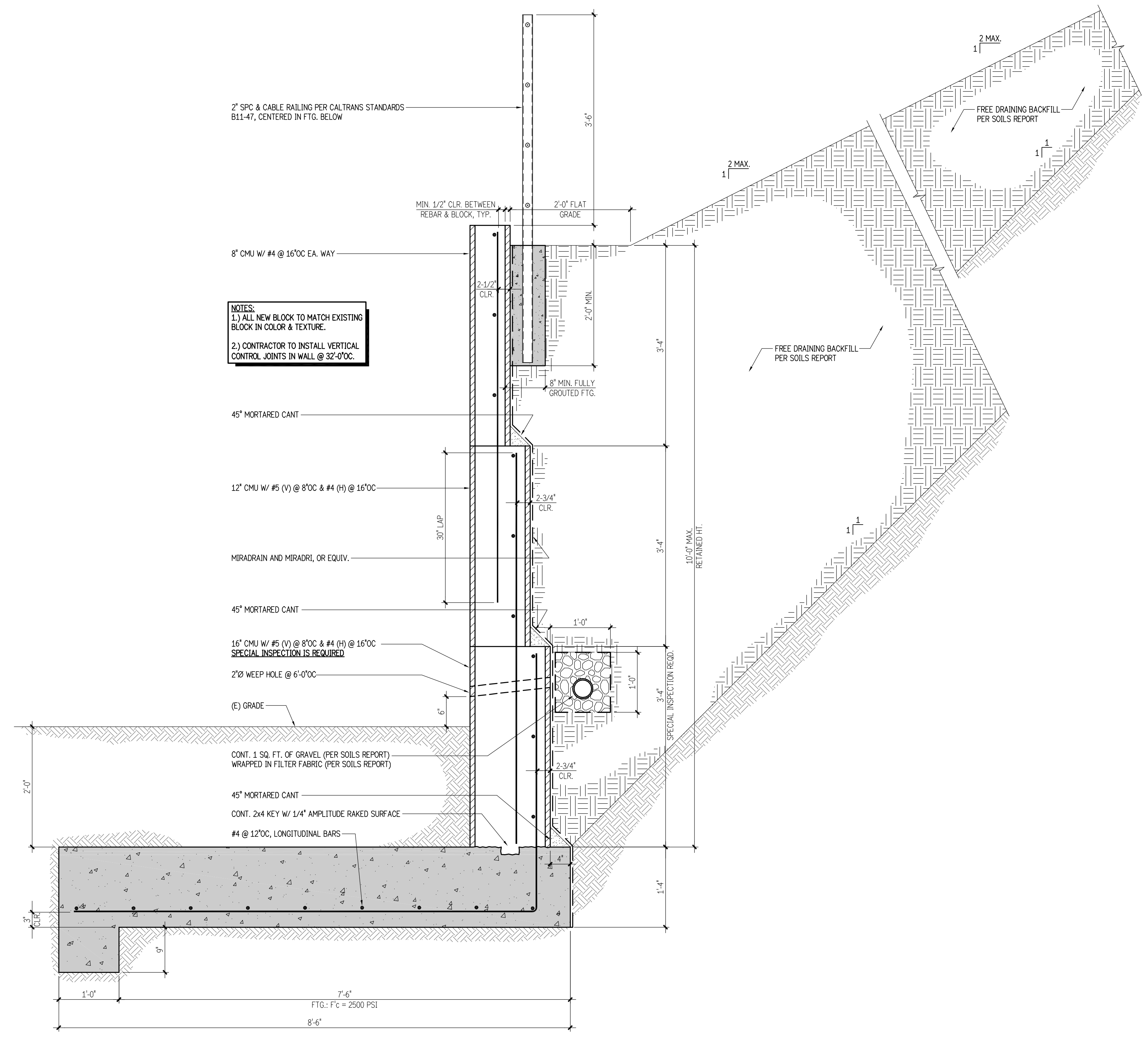
3 10'-0" RETAINING WALL 1'-1'-0"
